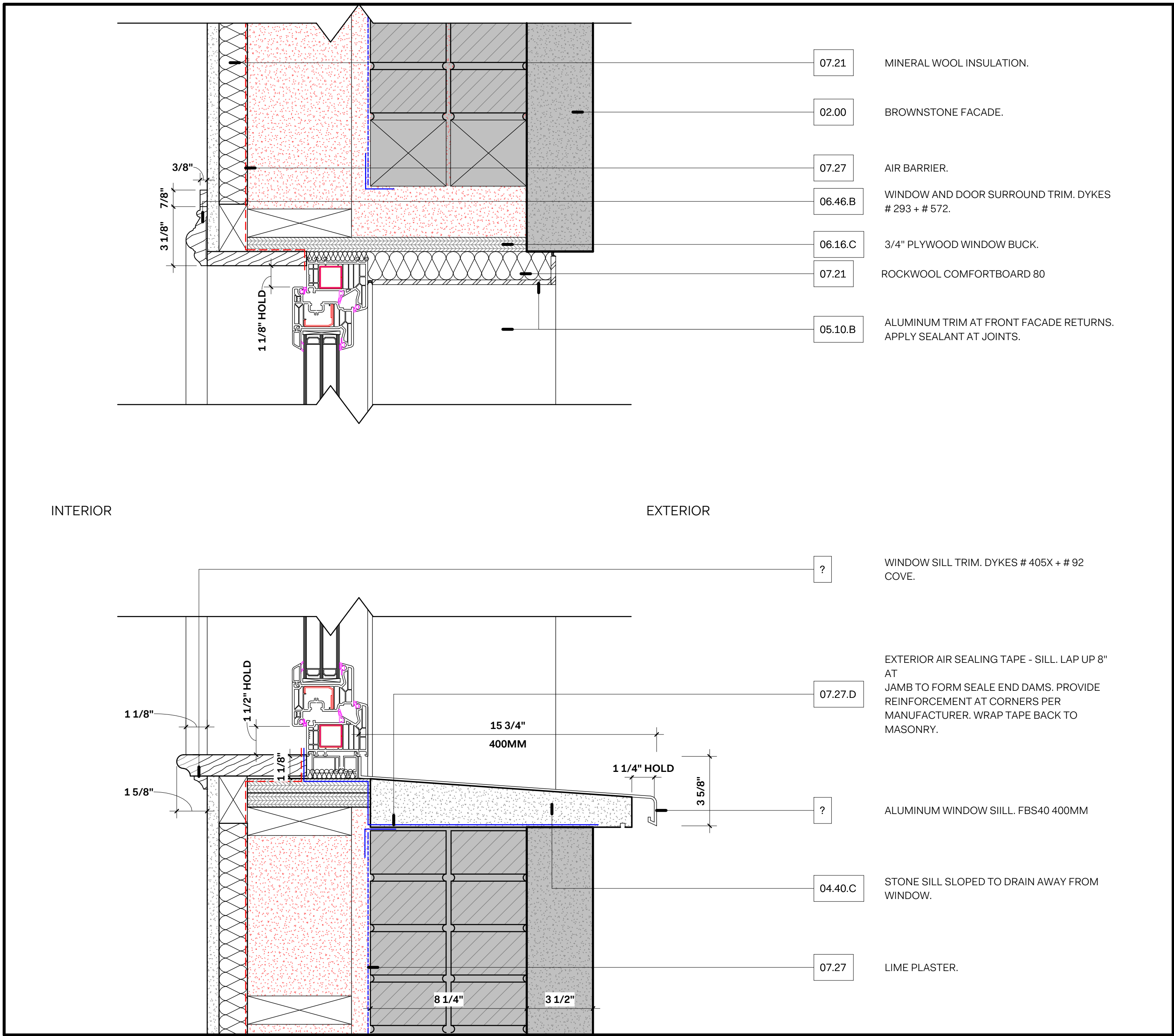
2 TYPICAL WINDOW - FRONT FACADE - HEAD/SILL 3" = 1'-0"
